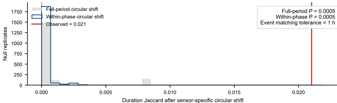
Limited temporal concordance between health and hard-availability events
