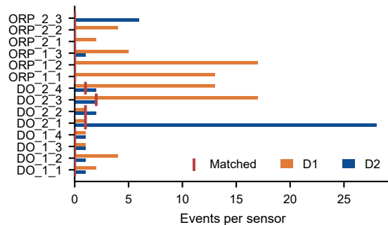
(b) Channel-level event counts
