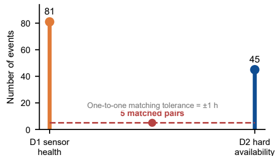
(a) Limited one-to-one event concordance
